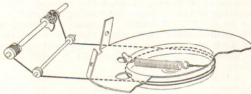
A typical drive cord arrangement
