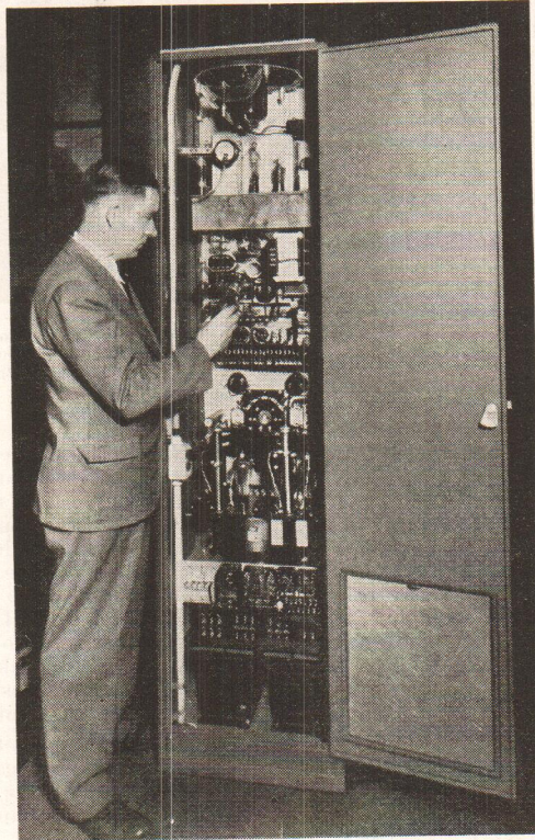
Inserting a tube in rear of the transmitter of Police Department at Newark. Photo, courtesy Western Electric Co.
