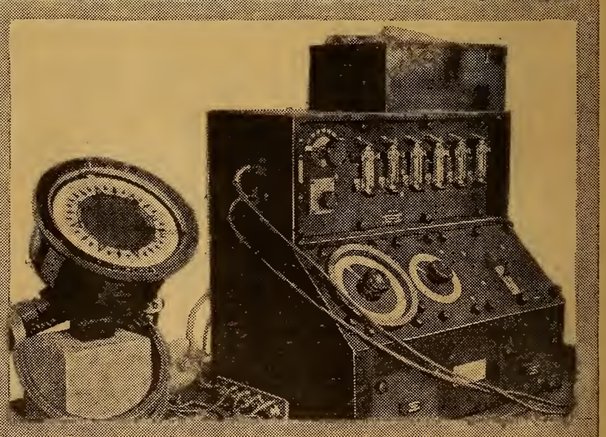
The seventh wonder of the maritime world, the "D. F." (direction finder) or Radio compass as it appears on the world's fastest liner, the S.S. Mauretania. The device consists of a Sperry gyro repeater and a special six-tube Radio receiving set. The D. F. is directly connected with the ship's compass ©K. & H.
