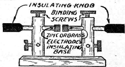
STATIONARY SPARK GAP FIG. 2
