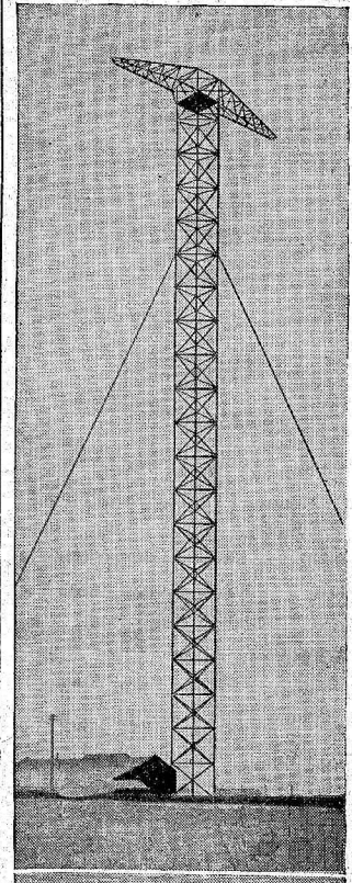
The Marconi Beam Radio station at Dorchester is completed and will get its first real tests during the international broadcast week, starting January 24. Great cast steel masts, as shown above, with cross-arms at the top on which the station's aerial and counterpoise are strung, are placed at intervals of 600 feet for a distance of more than a mile from the station. Building at base houses both the transmitting equipment and studio.
