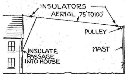
Figure 1. Typical aerial installation where mast supports one end.
