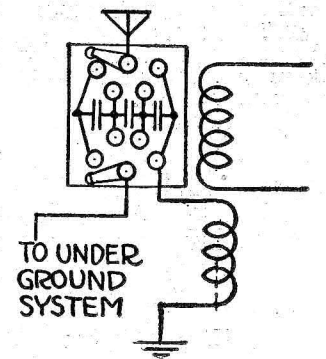
Figure 5. A selectivity switch worth making.
