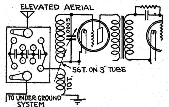
Figure 6. Here is suggested a method of coupling the input of buried antenna to your set.
