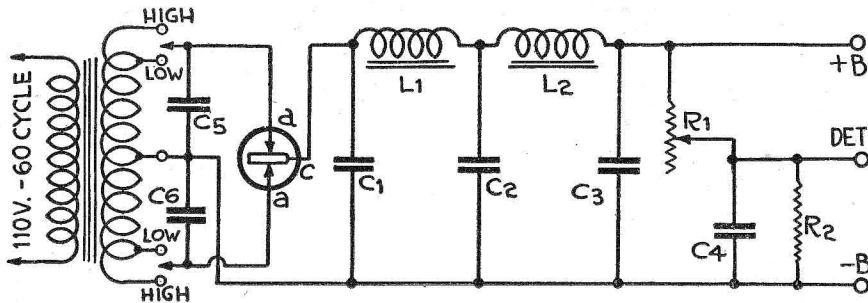
Figure 2. Circuit of Thordardson-Raytheon-Potter eliminator.
