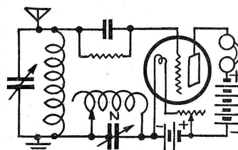
Figure 3. On first glance one might assume that this is a rejector circuit, but it isn't.
