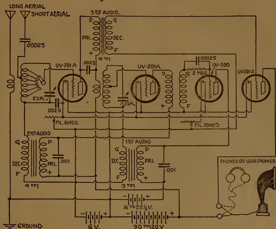
Figure 14—Tuned Radio and the Grimes Inverse Duplex
