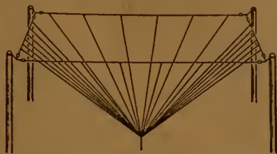
Figure 55—The four-fan antenna is unsurpassed in efficiency but difficult of erection
