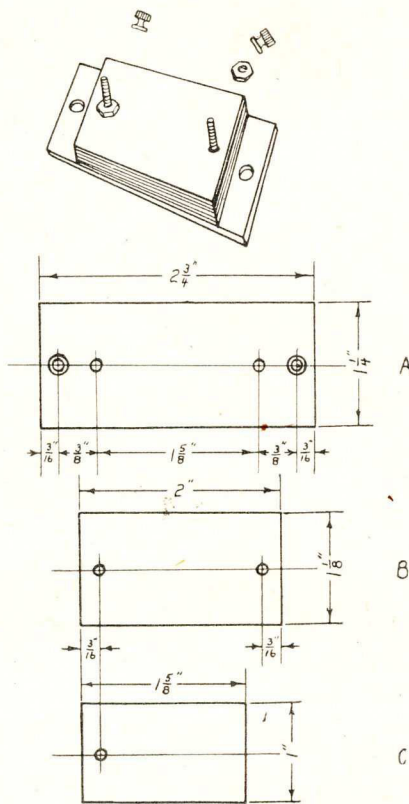
"A" is the bottom plate, "B" the top and "C" the thin copper strips. The mica plates are same size.
