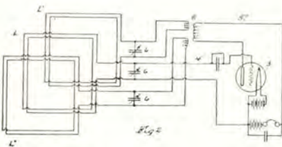
Multiple Regenerative Loop Antenna and Circuit
