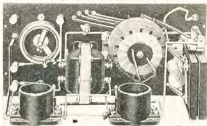
Rear view of Crosley 51 receiver, showing two-tube Armstrong regenerative hook-up. One multitap operates both tubes.
