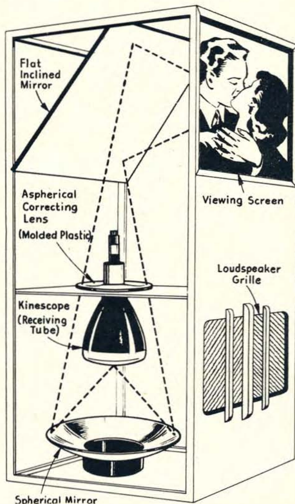
BROKEN LINES ON DIAGRAM indicate the path of light beams from cathode-ray receiving tube—to spherical mirror—through correcting lens—to flat mirror—and to final projection on the screen itself.
