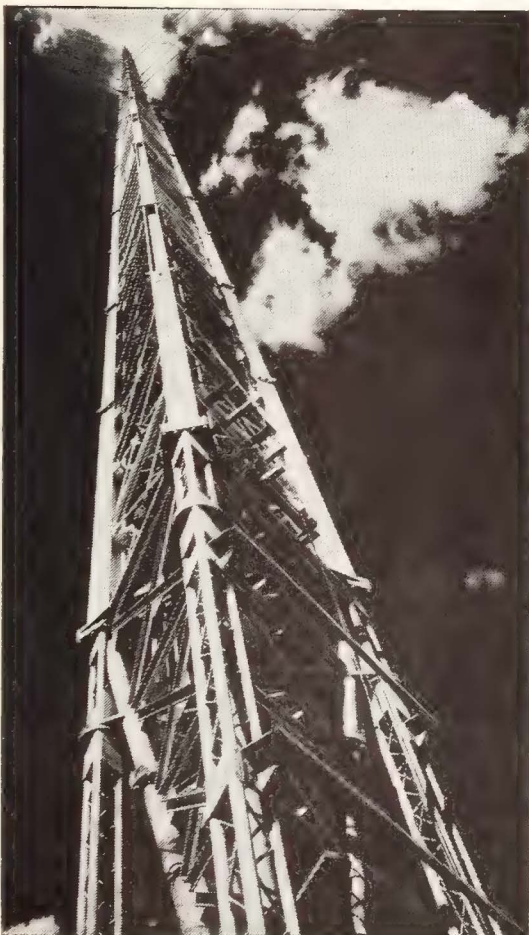
Tallest Structure In The World. This gigantic television tower belongs to station KWTW in Oklahoma City. It is 1572 feet high—100 feet taller than the very tip of the Empire State Building. To withstand the screaming 150 mph winds, most of the top sections were made from USS Man-Ten, a special high strength steel designed for demanding jobs.
